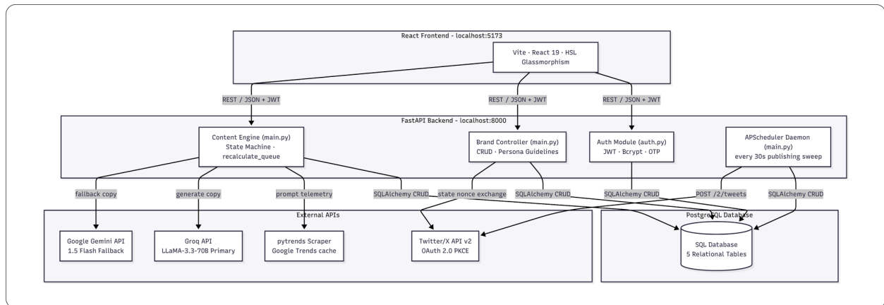
Figure 3.1: BrandOrbit Modular System Architecture Diagram
